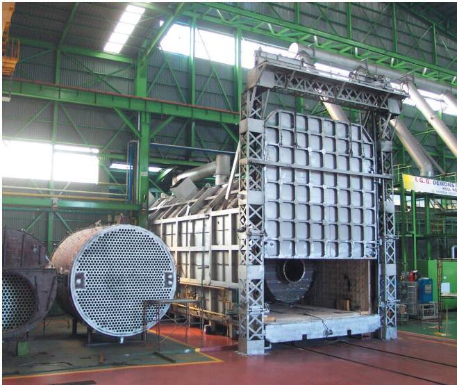
Large size annealing furnace
