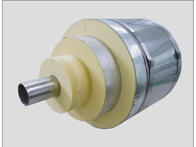
PIR/PUR Pipe Cover with SUS Jacketing
