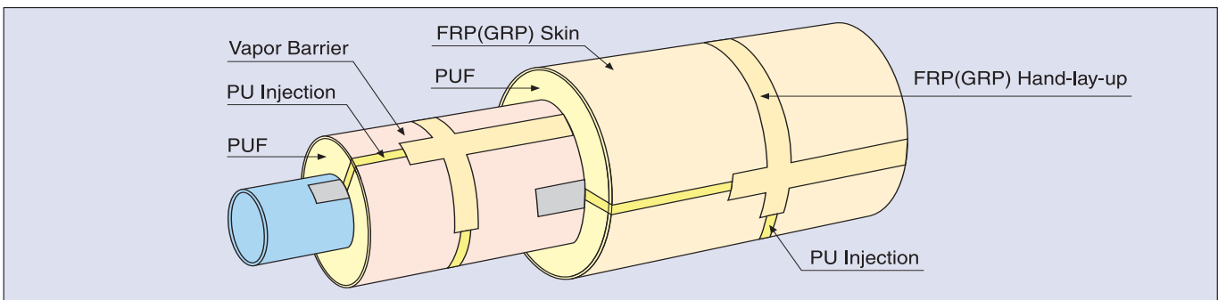
Insulation Construction
